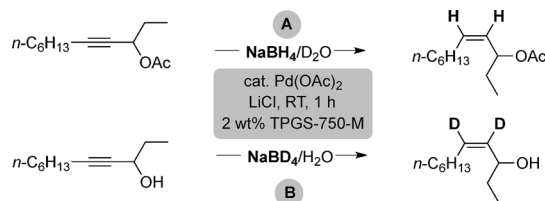
Scheme 7. Semihydrogenation with A) \text{NaBH}_4 in \text{D}_2\text{O} ; B) \text{NaBD}_4 in \text{H}_2\text{O} .
