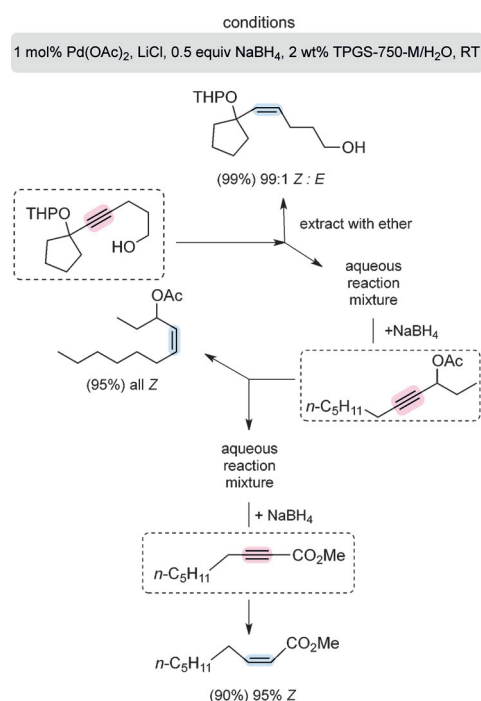
Scheme 5. Recycling of the aqueous reaction mixture using different starting materials (MTBE extraction).
